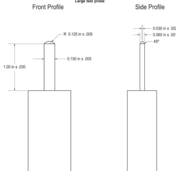
Figure 139.2 Large test probe
