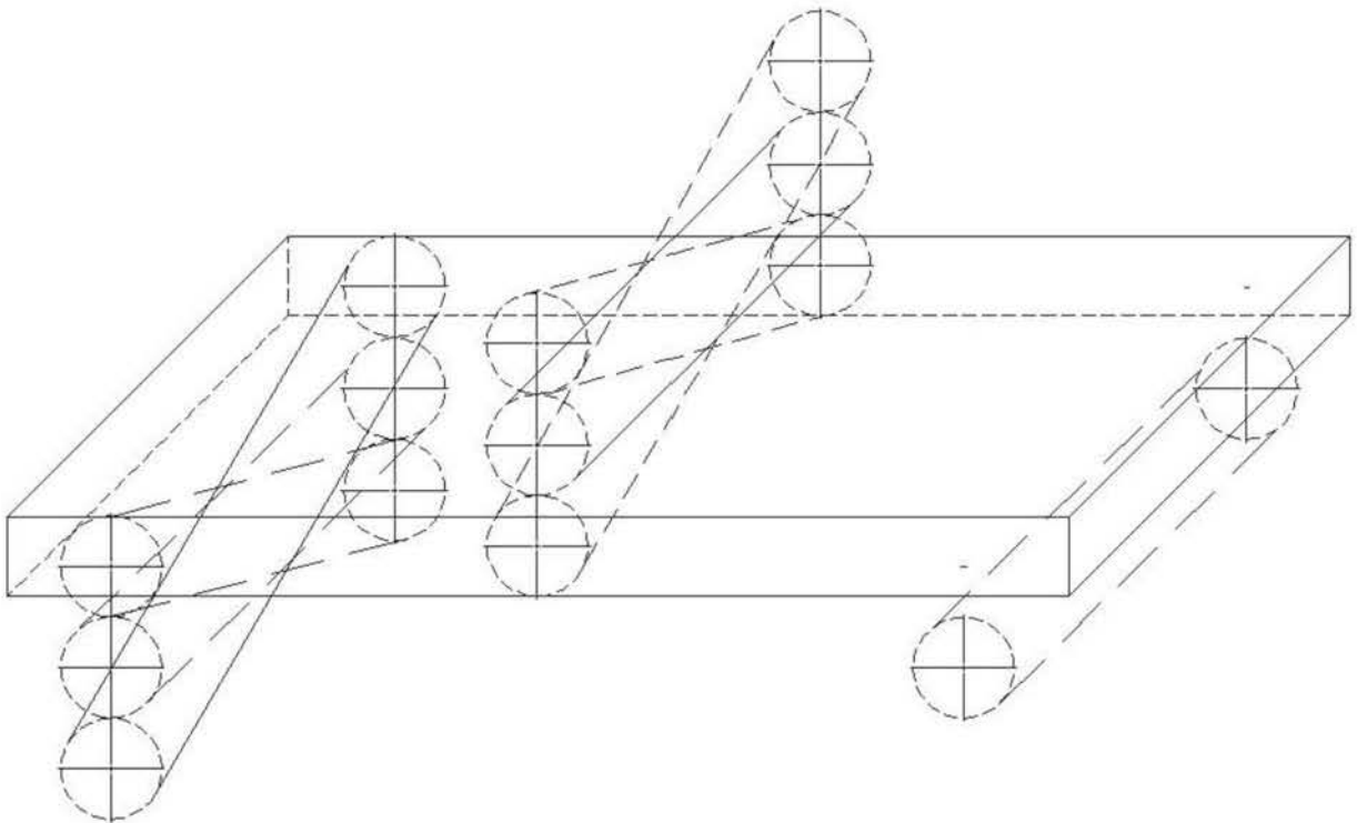
Figure 2 — Allowable movement of rods
